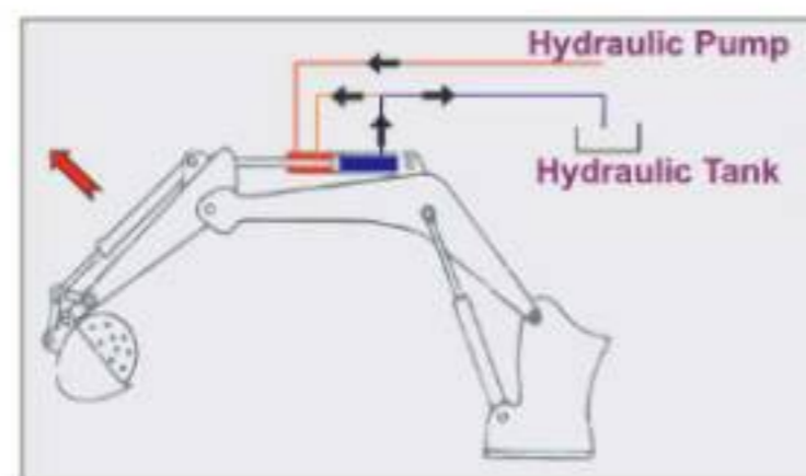
Regeneration System
